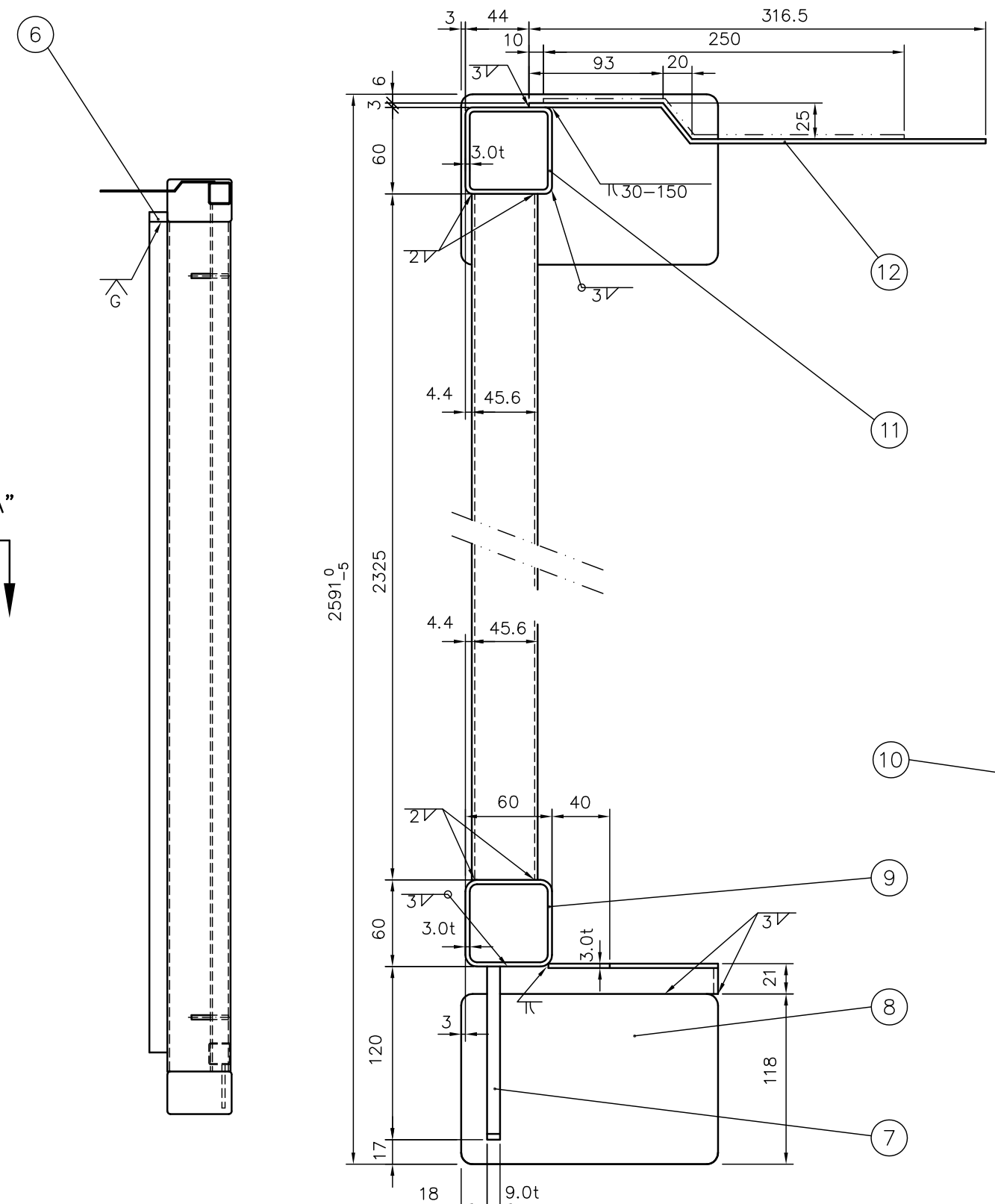
SECTION "B"-"B" 1:5
